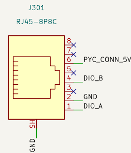
modular–jack
